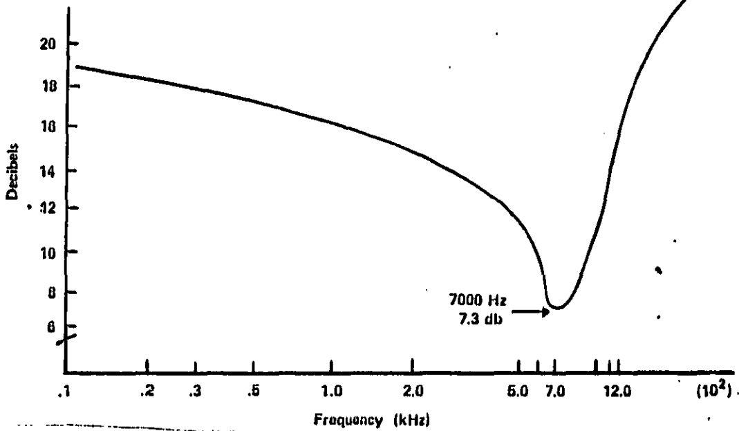
FIGURE 1. Auditory Threshold for Sheep. Plot of minimum auditory threshold with decibels shown as sound pressure level above background (26 dB). (Ames and Archart, 1972)
