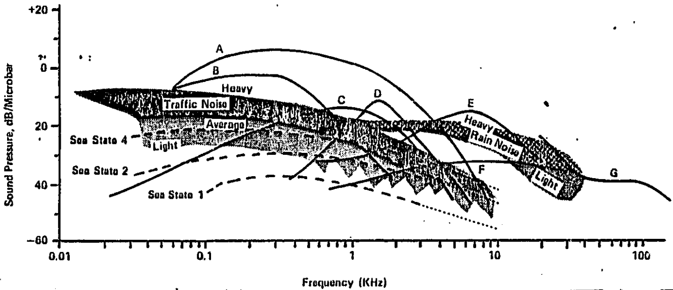
FIGURE 0. Shallow water (<70 m), ambient noise (spectrum level). Data have been extracted from numerous sources and redrawn. (Myrberg, 1980)
