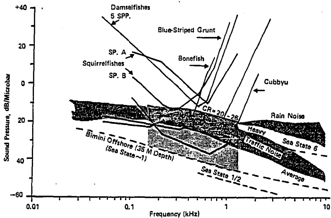
FIGURE 12. Low frequency ambient noise and its probable masking effect on the hearing abilities of selected marine fishes, whose peak sensitivities are found within that spectrum. The hatched area is the region chosen to show the amount of masking that would extend above the arbitrarily chosen level of ambient noise (in spectrum level). The ambient chosen was offshore the island of North Bimini, Bahamas where all the species reside. Audiograms were selected from various authors. (Myrberg, 1980)
