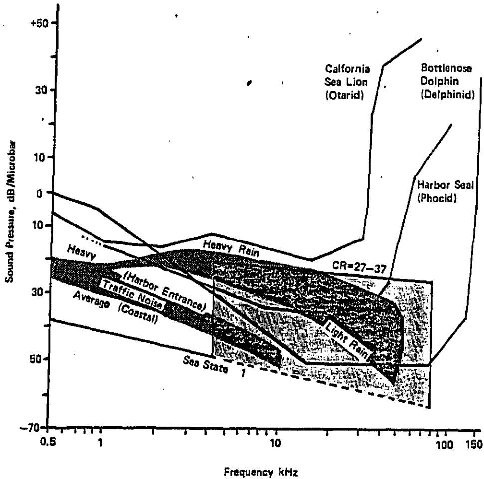
FIGURE 9. High frequency ambient noise and its probable masking effect on the hearing abilities of selected marine mammals whose peak sensitivities are found within that spectrum. Audiograms were redrawn from several authors. The hatched area is the region chosen to show the amount of masking that would extend above the arbitrarily chosen level of ambient noise (in spectrum level) with the critical ratios (CR) provided. (Myrberg, 1980)
