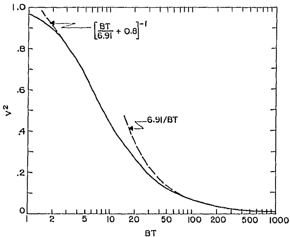
Figure 32. Normalized variance, (\langle p^2 \rangle^2 - \langle p^2 \rangle^2) / \langle p^2 \rangle^2 , where \langle \rangle denotes the average taken over all room locations, of the mean-squared sound pressure in a room having a reverberation time, T , and excited by random noise of bandwidth, B . The curve corresponds to eq. (85) which is valid for modal overlaps greater than about 3.
