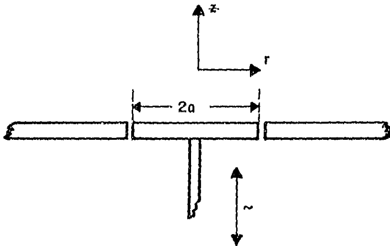
Figure 1B. Schematic representation of a rigid circular piston of radius, a , contained in an infinite baffle.
