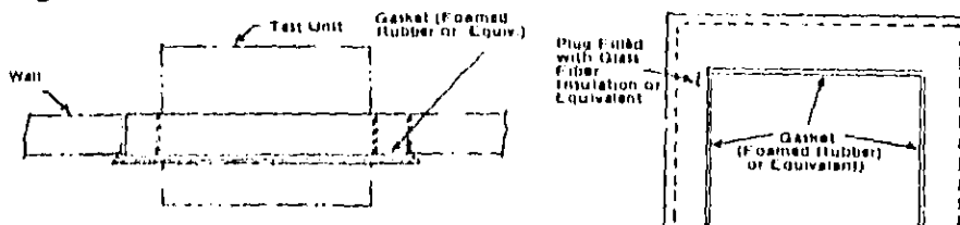
Fig. 3 Typical sound isolation plug
