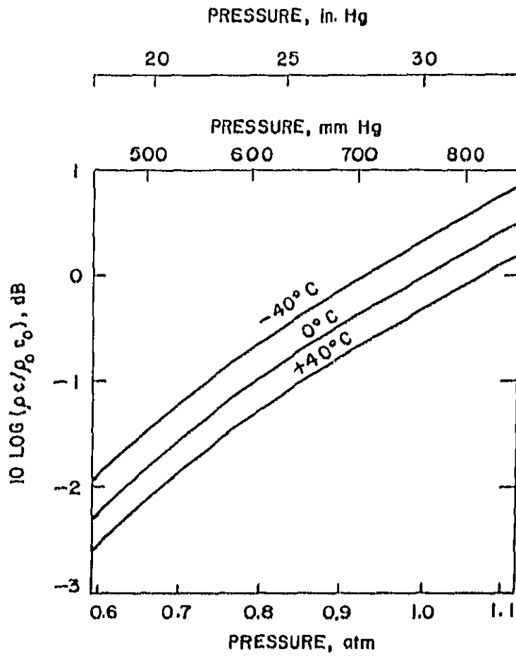
Figure 14. Pressure dependence of the acoustic resistance of air.
