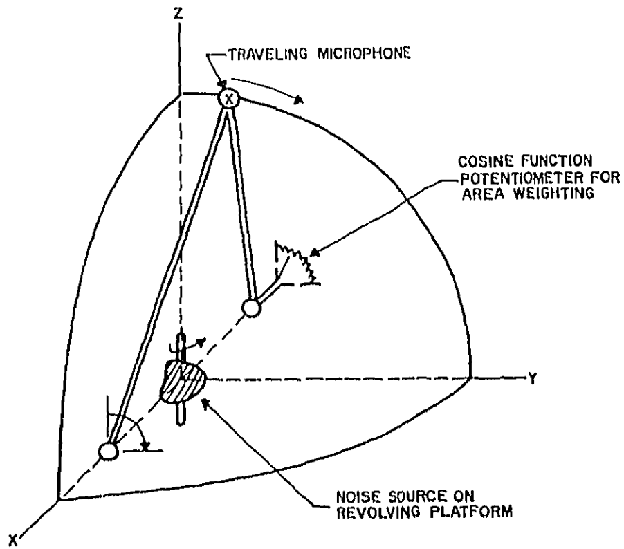
Figure 28. System for microphone traverses along meridional paths[14].
