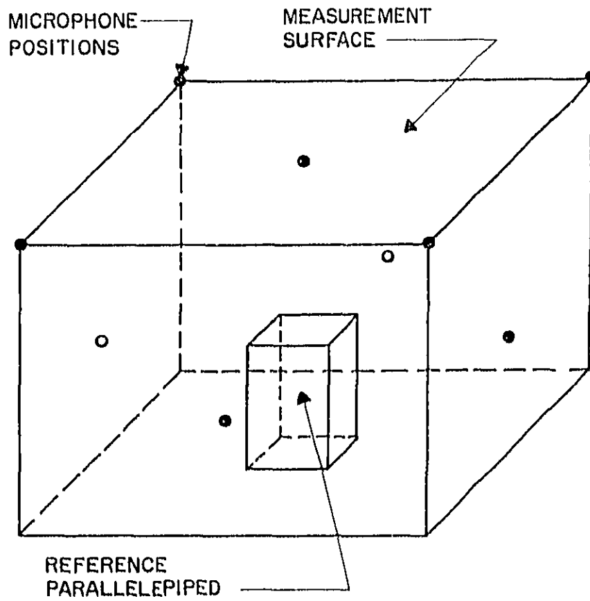
Figure 29. Microphone array for a parallelepiped measurement surface[13].
