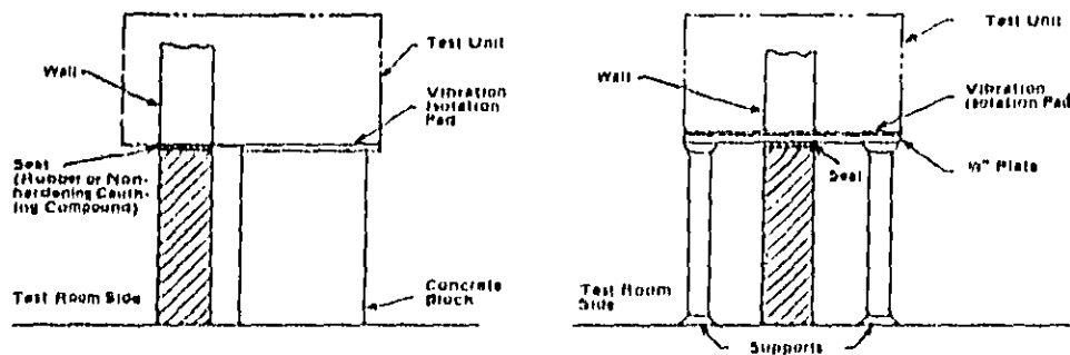
Fig. 2 Auxiliary mountings
