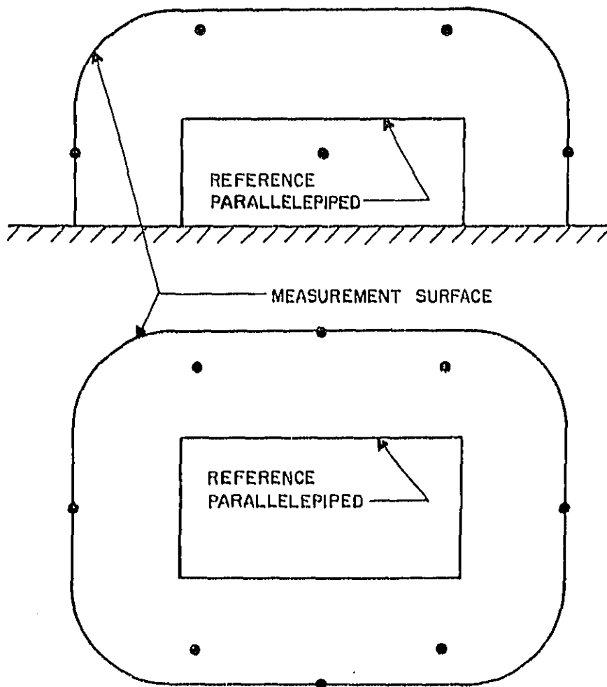
Figure 30. Microphone array for a "composed" measurement surface[13].
