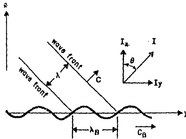
Figure 22. Schematic representation of sound radiation from an infinite plate in which there is a plane bending wave propagating at speed, c_B .
