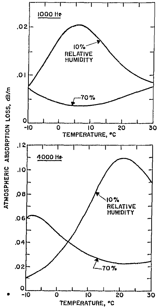
Figure 15. Atmospheric absorption loss in air as a function of temperature for relative humidities of 10 and 70 percent at frequencies of 1000 and 4000 Hz.
