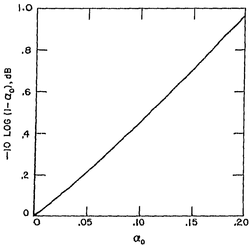
Figure 9. The effect of neglecting the 10 \log (1-\alpha_0) term in eq. (16).
