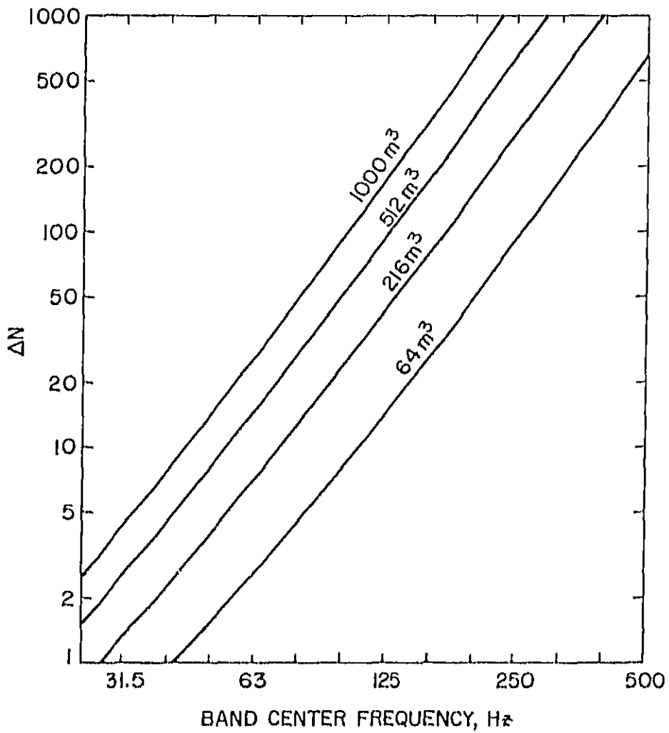
Figure 10. Approximate number of normal modes in a 1/3-octave frequency band for cubical rooms of the volume shown.
