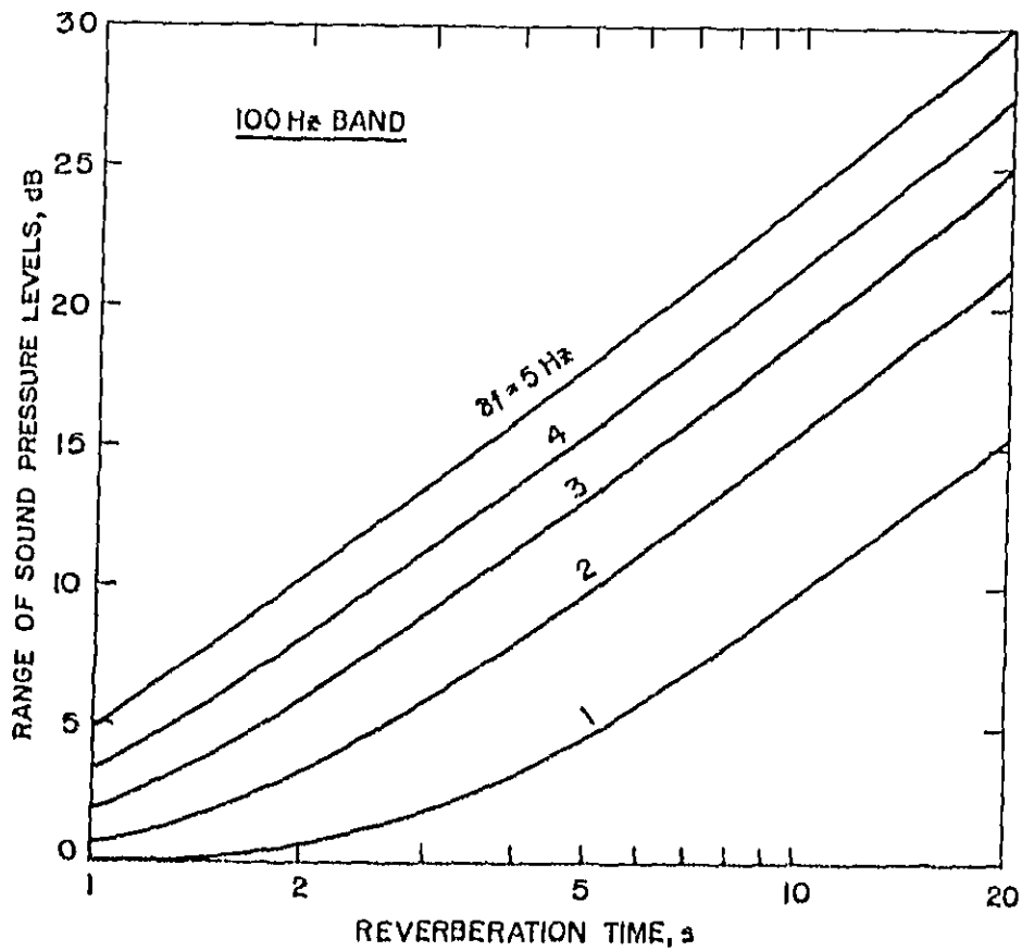
Figure 12. Range of the variation (peak-to-valley in Figure 11) in the frequency response of a reverberation room for frequencies near 100 Hz as a function of reverberation time for different modal spacings.
