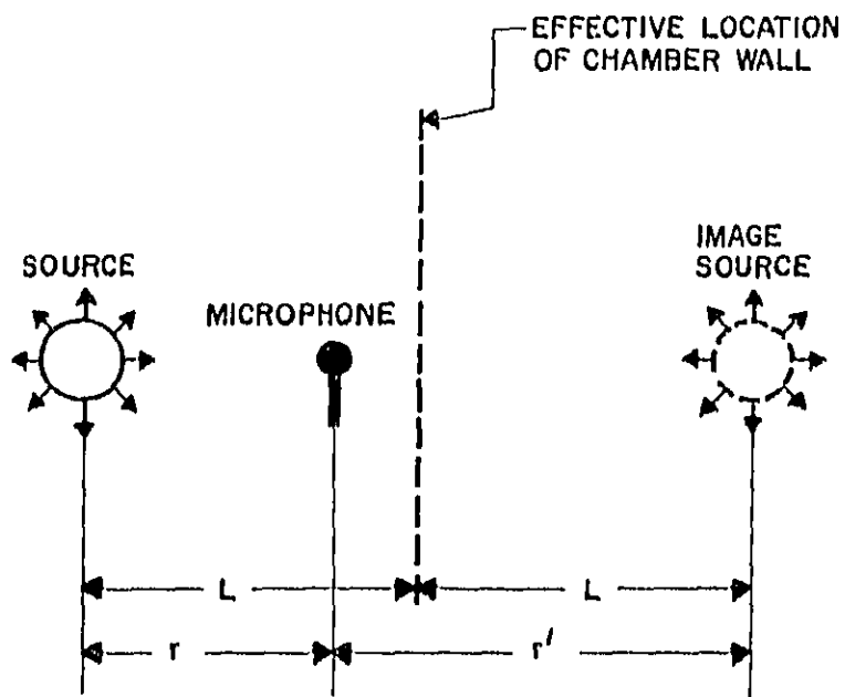
Figure 3. Schematic representation of a sound source in an anechoic chamber. The sound field produced by a source and its "image" only approximately represents the actual sound field.
