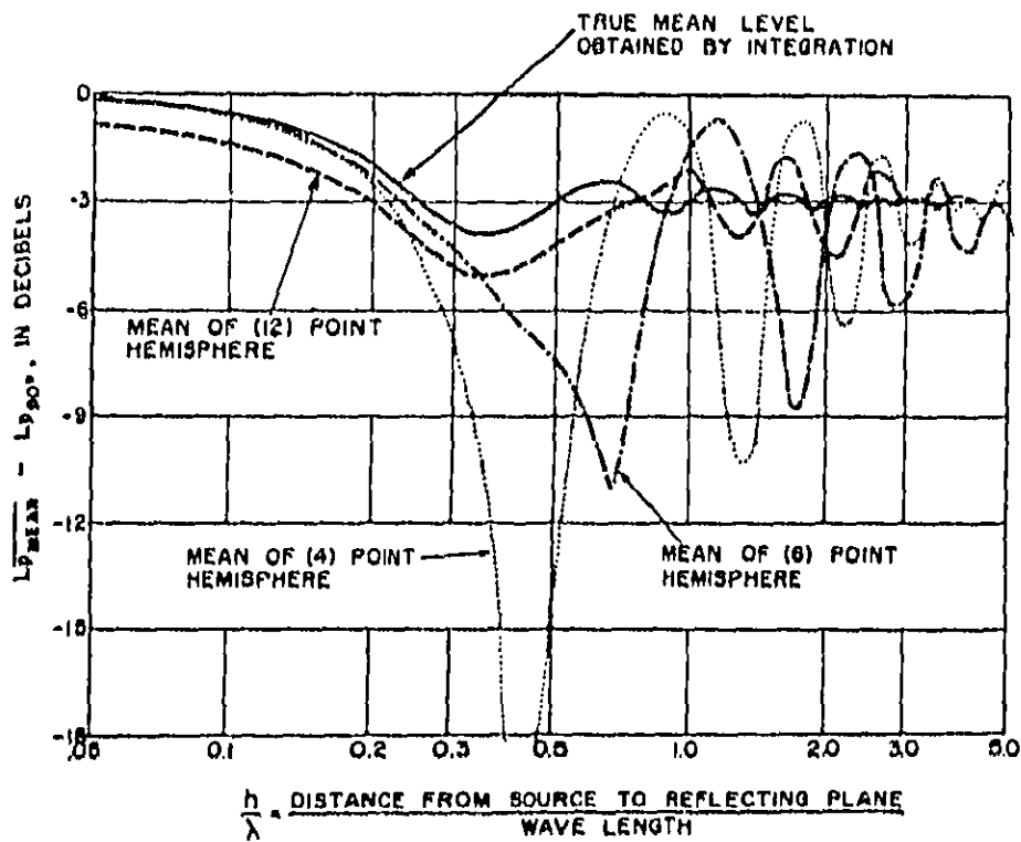
Figure 27. Error introduced by limited number of measuring points when determining sound power output of a random point source near a reflecting plane [73-74]. The error is the difference between the curve corresponding to a given microphone array and the solid curve which corresponds to the true mean level. All curves correspond to a 1/3-octave band width.
