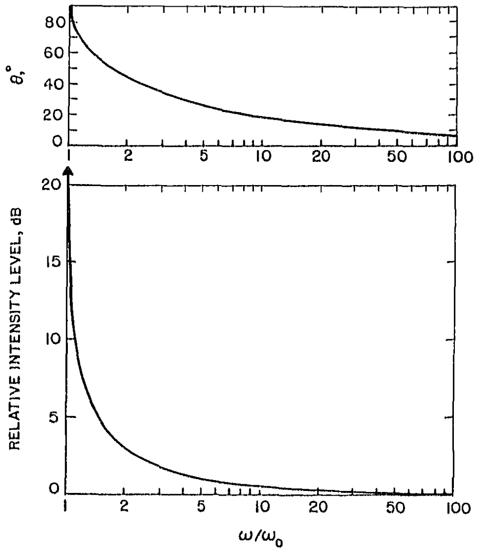
Figure 23. Far-field intensity level (lower figure) above the critical frequency for an infinite plate in flexure. The upper figure shows the direction (relative to the plane of the plate) in which sound is radiated.
