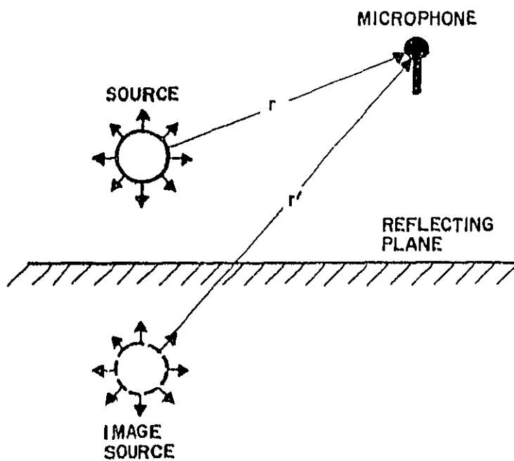
Figure 6. Schematic representation of a sound source in a free field above a reflecting plane.
