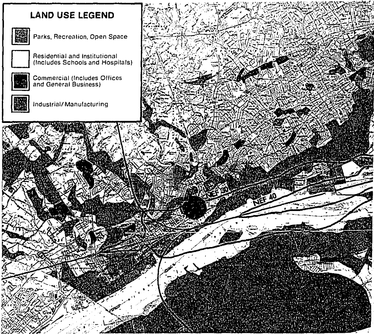
FIGURE PHL-2 PHILADELPHIA INTERNATIONAL AIRPORT 1978 NOISE EXPOSURE FORECAST FORECASTED BASELINE AIRCRAFT 4 CONCORDE OPERATIONS DAILY CONCORDE TAKEOFFS USE 3% G
