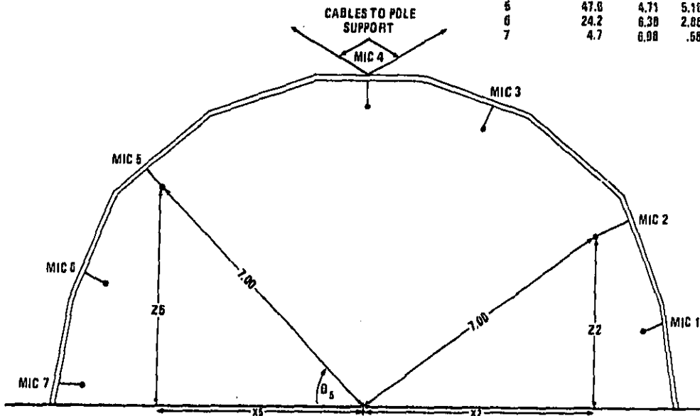
Figure 5 Far-field measurement array
