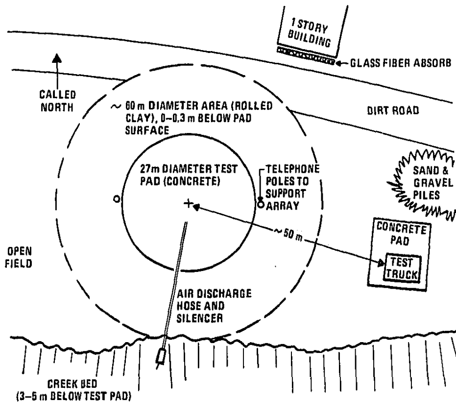
Figure 1 Field test site
