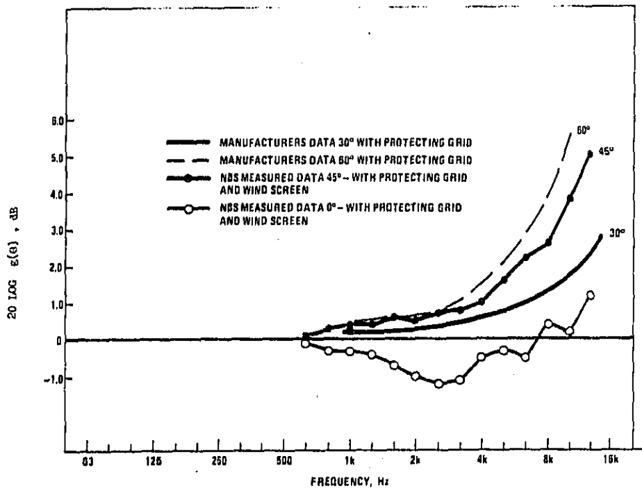
Figure 7 Microphone correction factor (Type 4145 cartridge)
