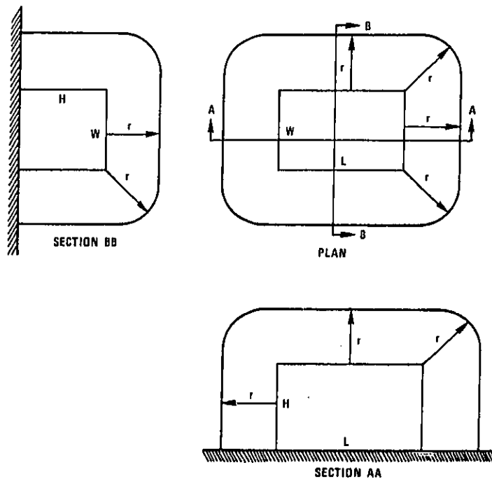
Figure 8 Conformal surface at a distance r from a rectangular box
