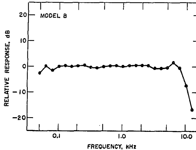
Figure 4.2-1. Relative frequency response of microphone.
