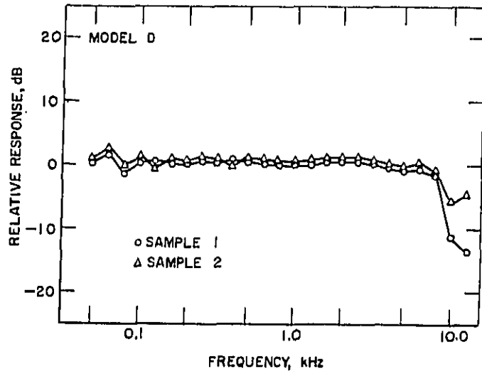
Figure 4.4-1. Relative frequency response of microphone.
