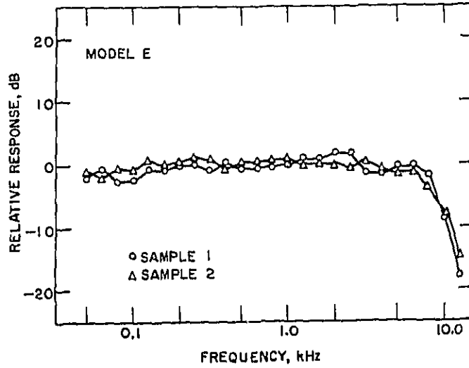
Figure 4.5-1. Relative frequency response of microphone.
