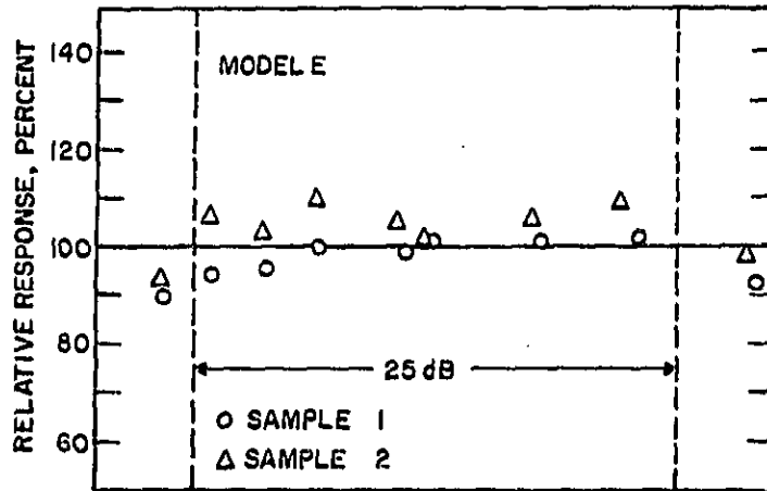
Figure 4.5-5. Relative response of noise exposure meter to an electrical signal covering a range of approximately 25 dB. See text for method of normalization.
