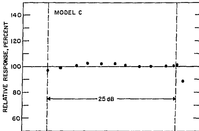
Figure 4.3-5. Relative response of noise exposure meter to an electrical signal covering a range of approximately 25 dB. See text for method of normalization.
