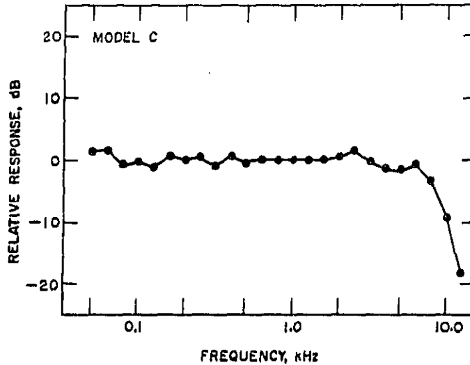
Figure 4.3-1. Relative frequency response of microphone.
