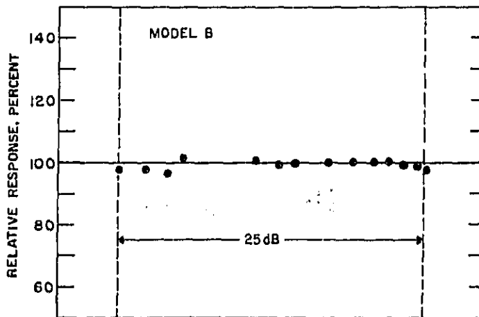
Figure 4.2-5. Relative response of noise exposure meter to an electrical signal covering a range of approximately 25 dB. See text for method of normalization.
