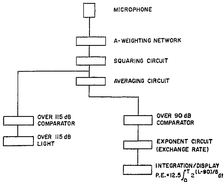
Figure 1. Block diagram showing the principle of operation for a typical noise exposure meter.
