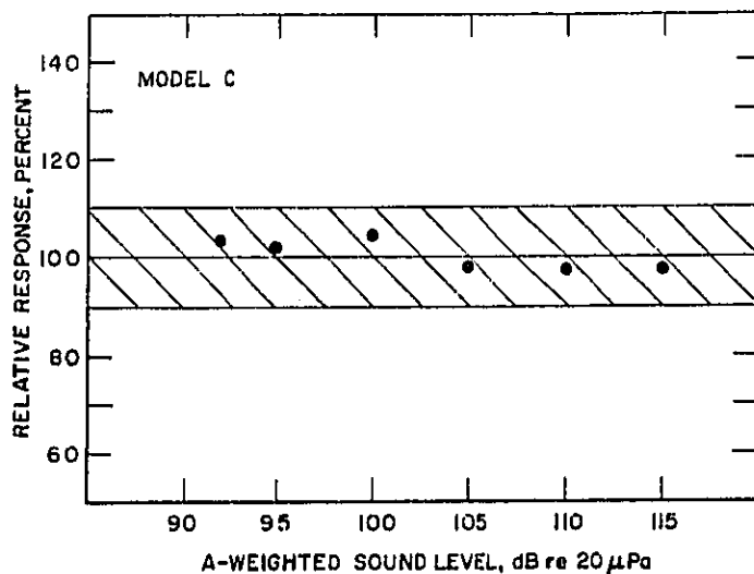
Figure 4.3-2. Response of noise exposure meter, relative to expected response, when placed in a field of pink noise (see text) at A-weighted-sound level from 92 to 115 dB.
