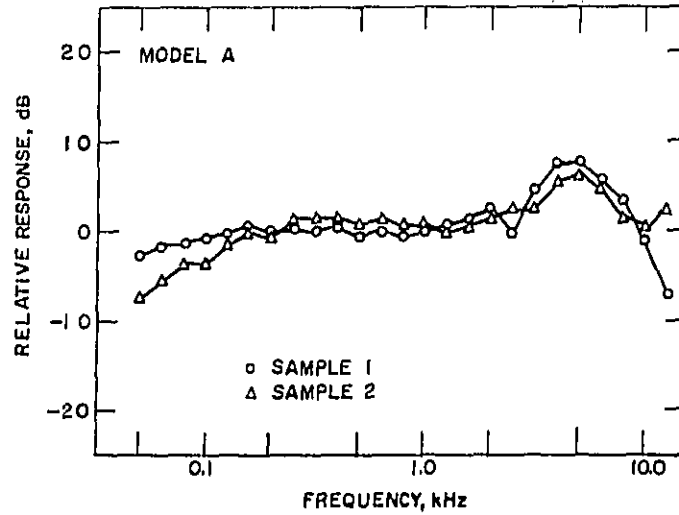
Figure 4.1-1. Relative frequency response of microphone.
