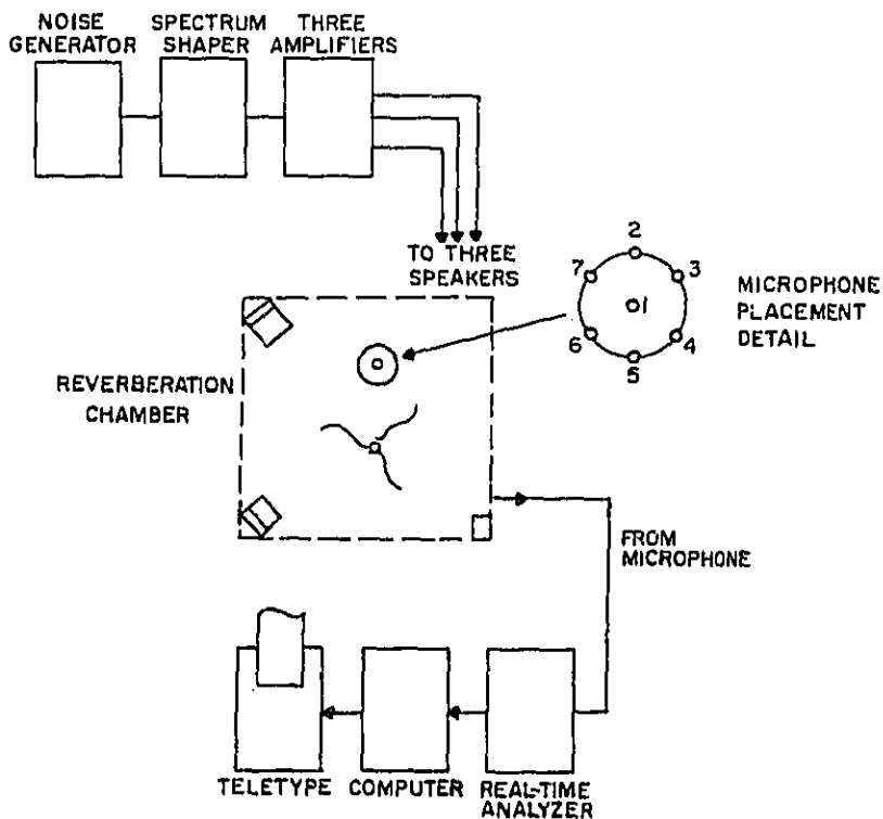
Figure 2. Block diagram of equipment used for acoustic tests in a reverberation chamber.
