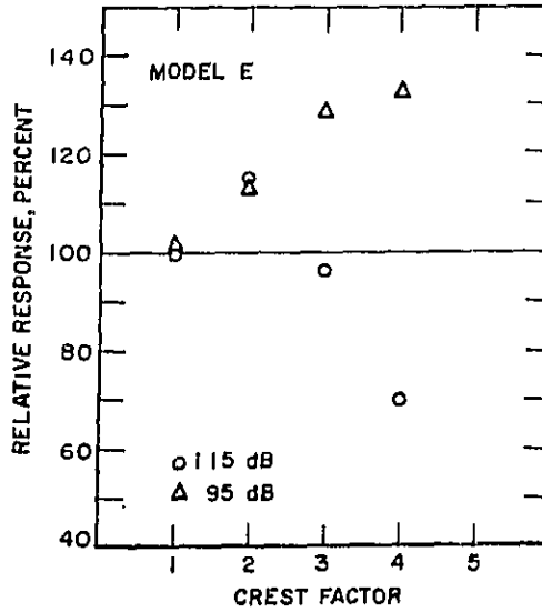
Figure 4.5-4. Response of noise exposure meter, normalized to 100% for a sine wave input, as a function of crest factor.
